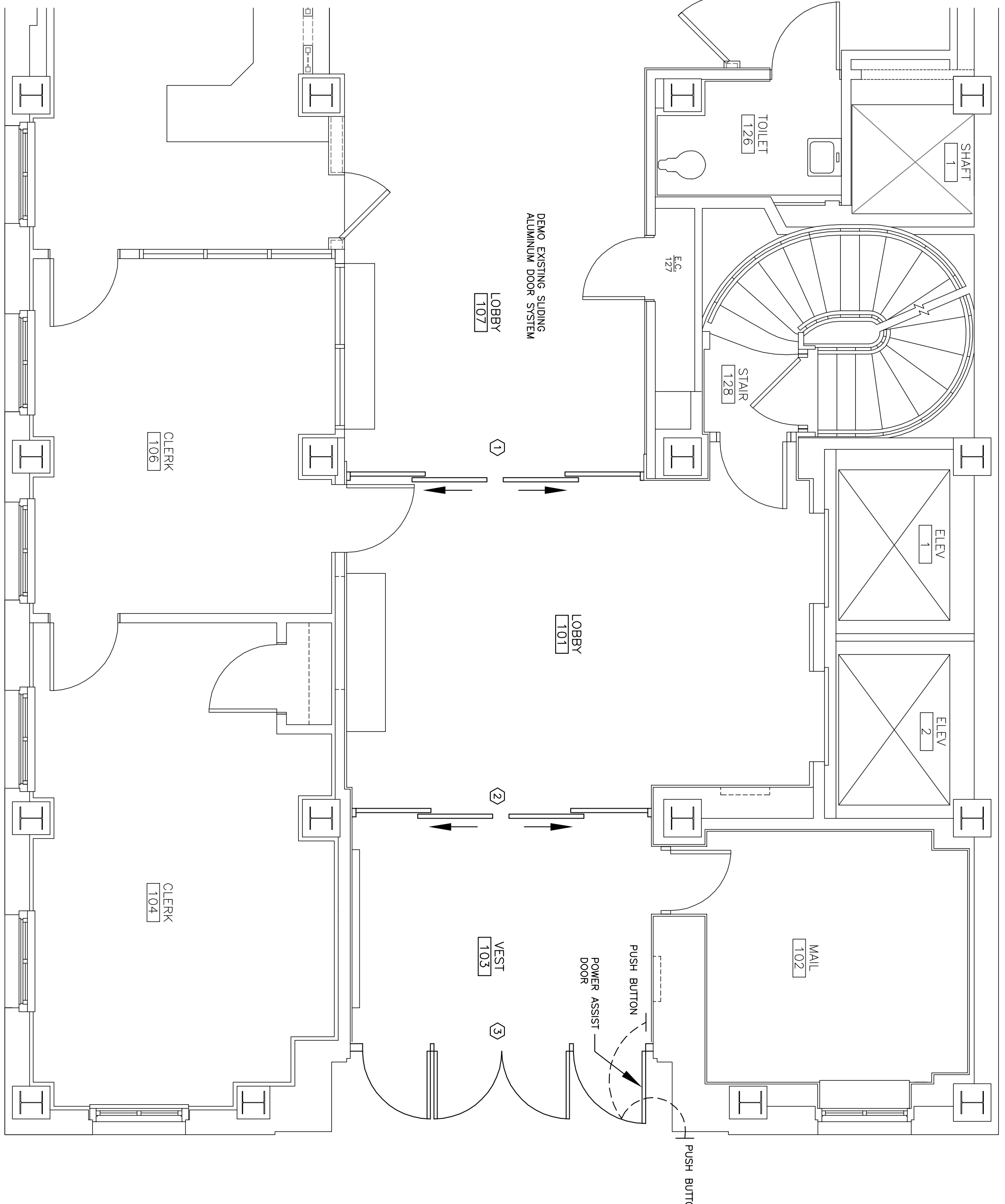
FLOOR PLAN 1/4" = 1'-0"
